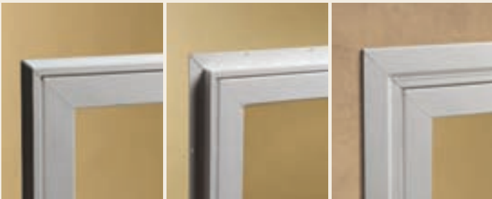
BLOCK Enables quick "tilt-in" installation with almost no disruption to siding or interior trim casework. NAILING FIN Perfect for home additions and remodeling where siding is removed. Available in 1-1/4" and 2" nail-fin widths, with a 1-3/8" setback. Z-BAR™ Makes replacing windows on stucco homes fast and easy, eliminating the need for costly repairs. Milgard Z-bar options provide an integral window trim and are available in standard and wide width options.
