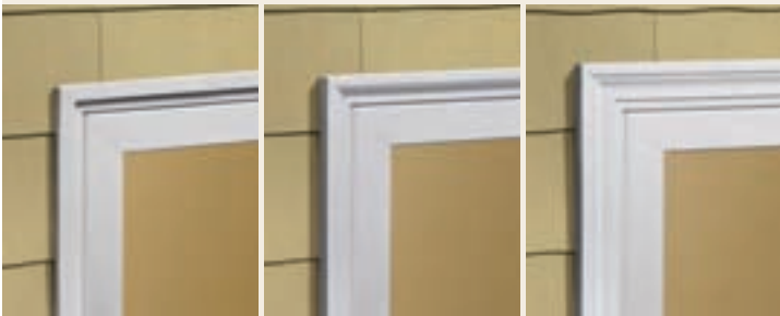
3/4" FLAT J-CHANNEL 1" CONTOUR J-CHANNEL 2" BRICKMOLD J-CHANNEL Choose from 3 decorative trim options to visually enhance homes with brick or lap siding exteriors. J-Channel options require a 2" nail-fin frame.
